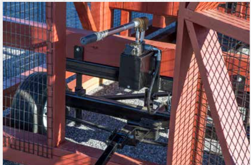
Shown with pump handle attached which will lift the coop up to 6 in. When not in use, handle can be removed and attached to inside of door.
